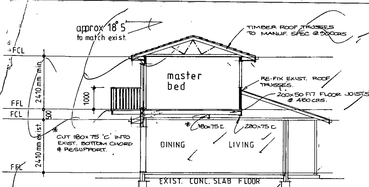
Section X-X
