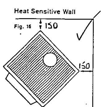
Corner Installation
