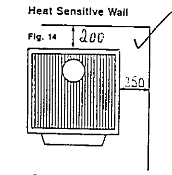
Standard Installation SINGLE FLUE SHIELD
