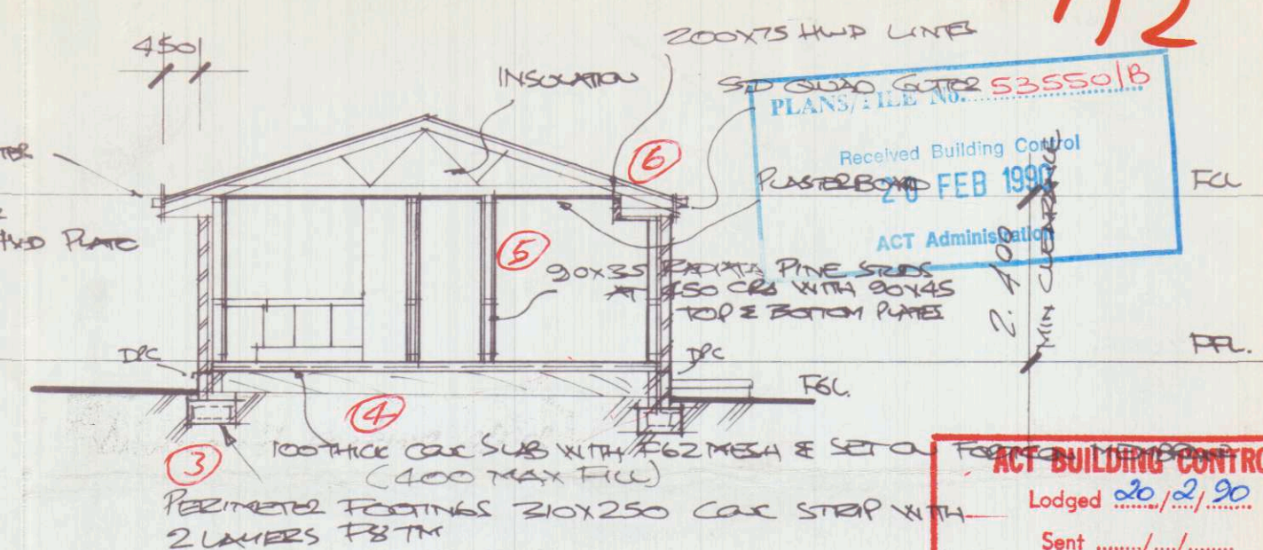
TYPICAL SECTION 1:100
