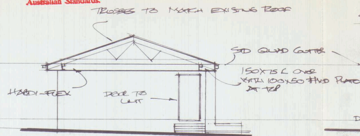
BREEZWAY SECTION 1:100
