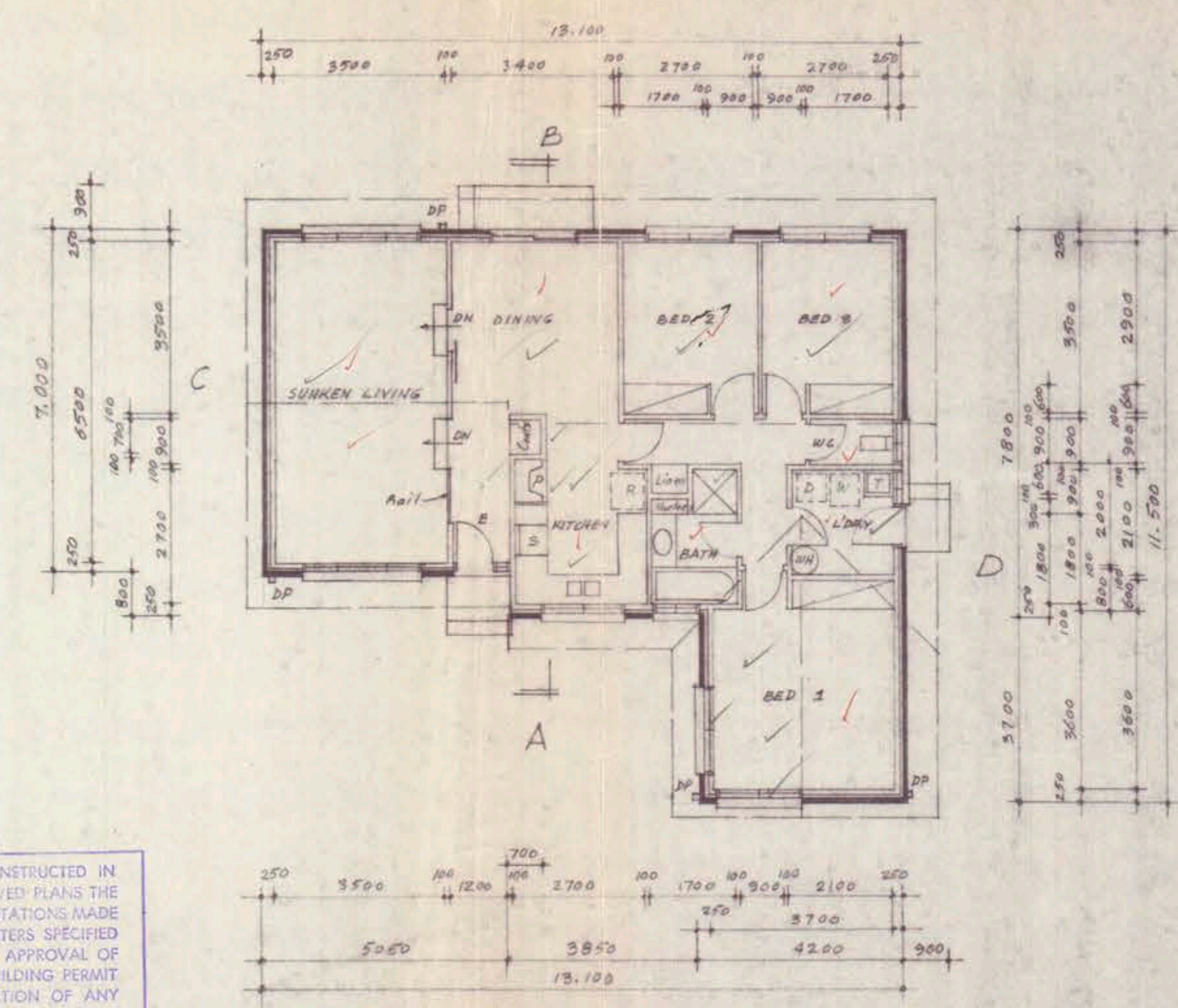
FLOOR PLAN
