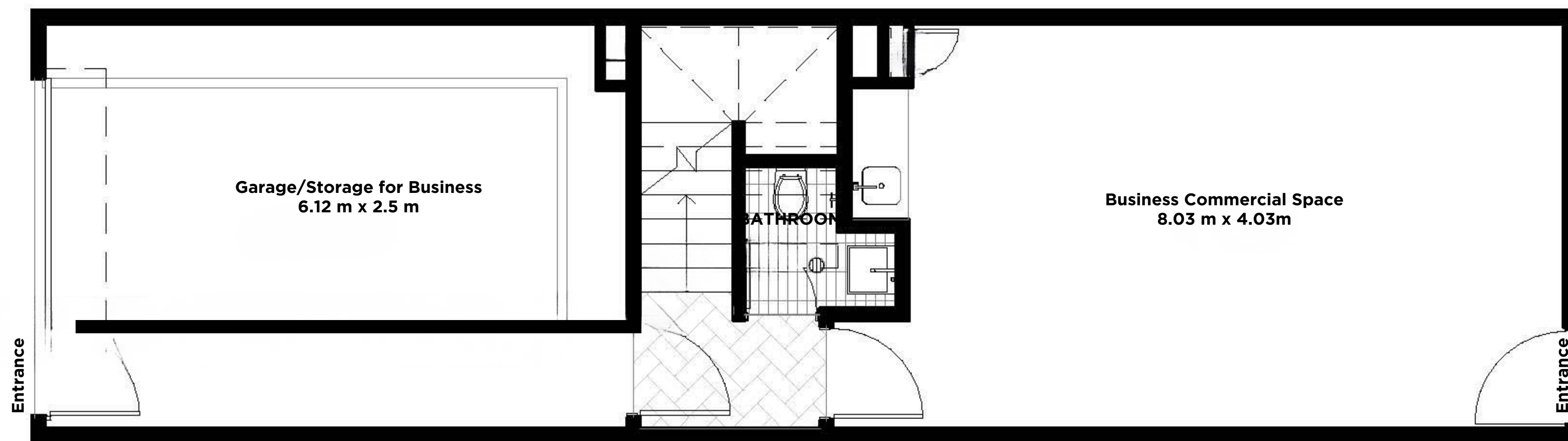
Ground Floor
