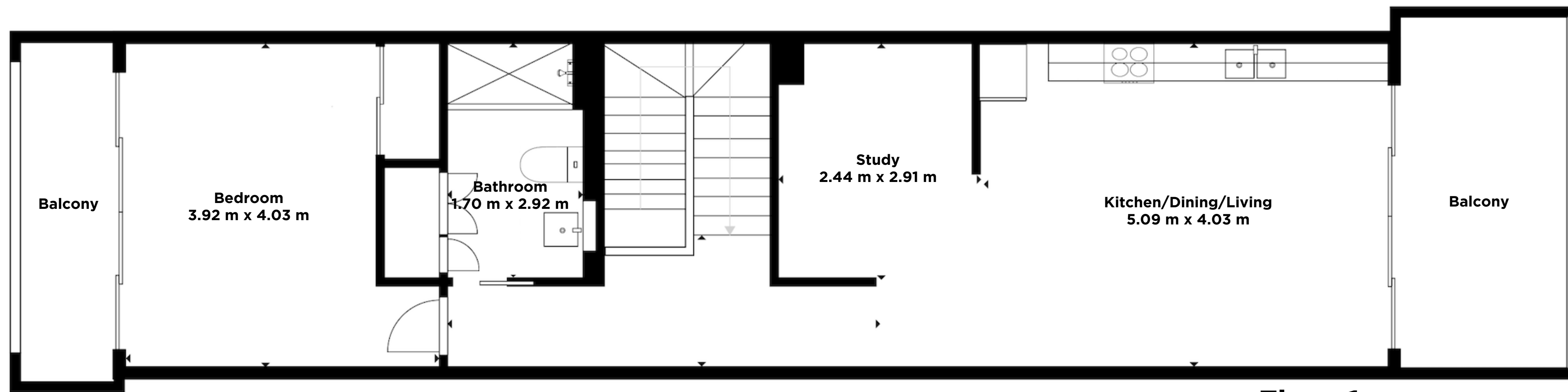
Floor 1
